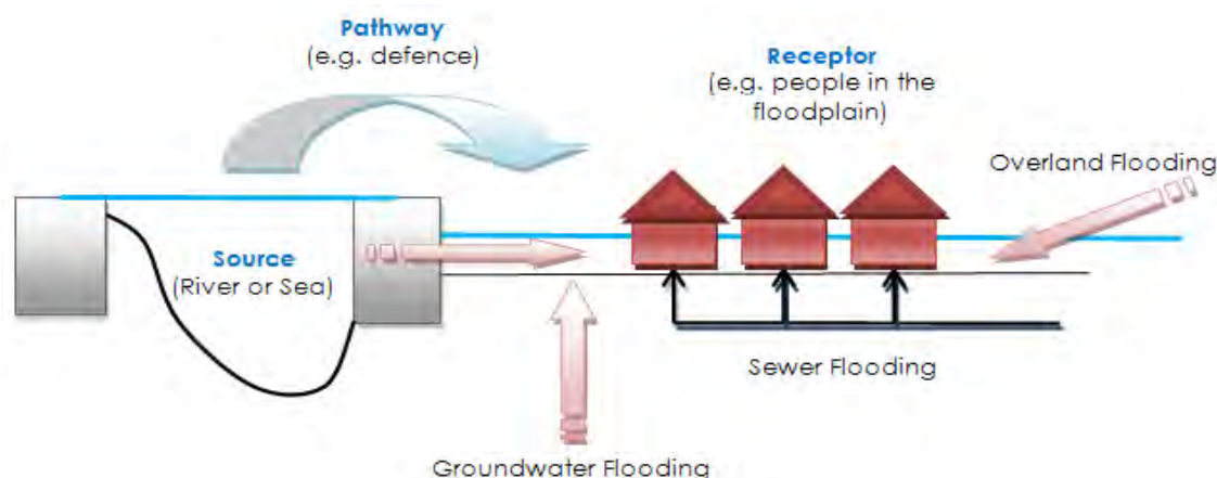
Figure 4-1 Source-Pathway-Receptor Model
